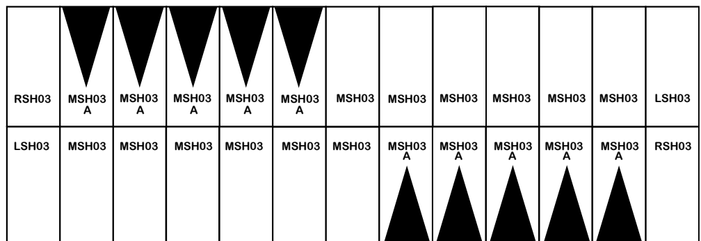
19.5' W x 7' L x 3" H Speed Hump w/Arrow Chevrons
